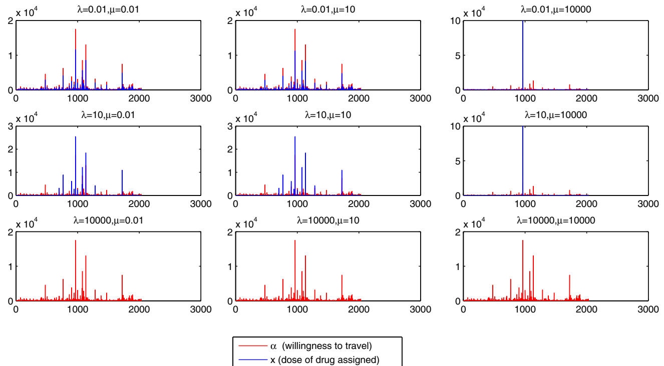
Fig. 4 Dynamics of pharmacies' access with varying lambda ( \lambda ) and mu ( \mu ) from 0.01 to 10,000. When lambda and mu are small in sub-graph a, many pharmacies are chosen for drug assignment. As for the
