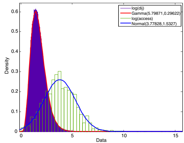
Fig. 3 Density distribution of access for each pharmacy and distance between two pharmacies
