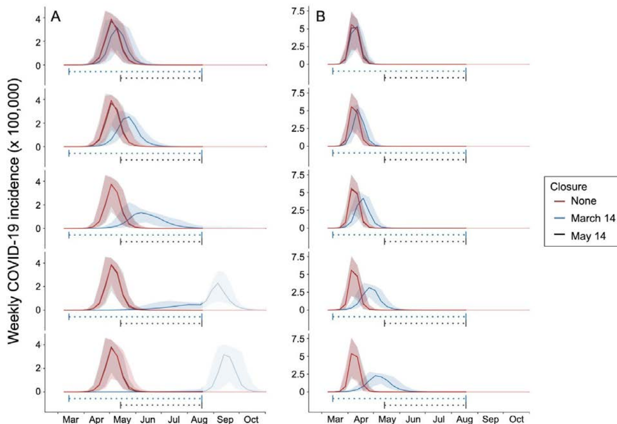
Appendix Figure 3. Projected weekly incident COVID-19 cases in the Austin-Round Rock MSA. Graphs show simulation results for different levels of social distancing and implementation times, assuming R_0 = 3.5 and an epidemic doubling time of A) 7.2 days (19–22) or B) 4 days (22,24,25). Each graph displays 3 projections: a baseline assuming no social distancing (red), social distancing implemented March 14–Aug 17, 2020 (blue), and social distancing implemented May 14–Aug 17, 2020 (black). From top to bottom, the graphs in each column correspond to increasingly stringent social distancing measures: school closures plus social distancing that reduces nonhousehold contacts by 0%, 25%, 50%, 75%, or 90%. Solid lines indicate the median of 100 stochastic simulations; shading indicates the inner 95% range of values. The horizontal dotted lines beneath the curves indicate intervention periods. The faded mid-August to December time range indicates long-range uncertainty regarding COVID-19 transmission dynamics and intervention policies.
