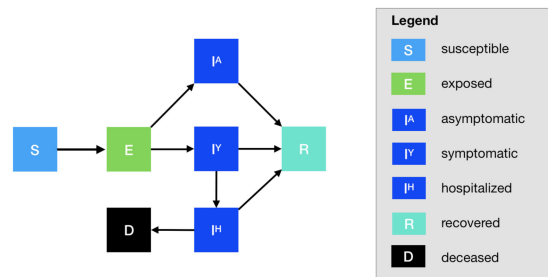
FIGURE 1. Compartmental model of COVID-19 transmission in a U.S. city. Each age and risk subgroup is modeled with a separate set of compartments. Upon infection, susceptible individuals (S) progress to the exposed (E) compartment and then to either symptomatic infectious ( I^Y ) or asymptomatic infectious ( I^A ) compartments. All asymptomatic cases eventually progress to a recovered class where they remain protected from future infection (R); symptomatic cases are either hospitalized ( I^H ) or recover. Mortality (D) varies by age group and risk group and is assumed to be preceded by hospitalization. Used, with permission, from Wang et al. 5-7
